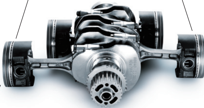
Horizontally opposed layout of the SUBARU BOXER engine
